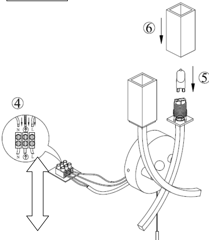
Wiring Details
